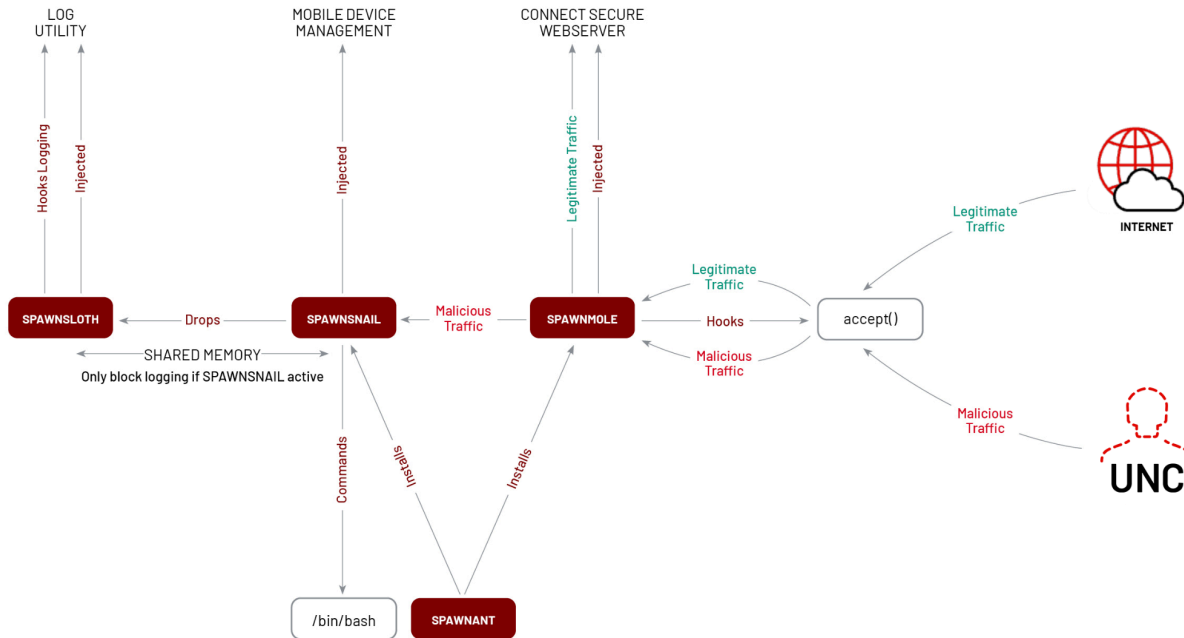
Figure 1: SPAWN malware family diagram
